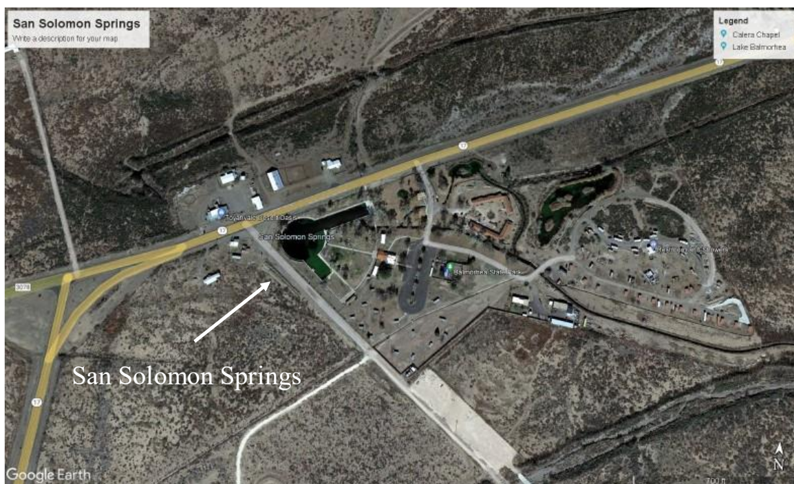
Enlarged view on Solomon Springs (from Google Earth)
