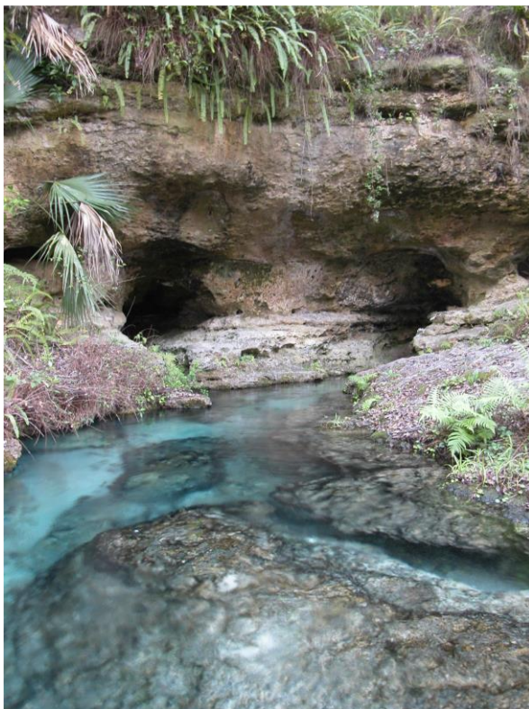
Rock Spring vent (Photo by FGS staff)
