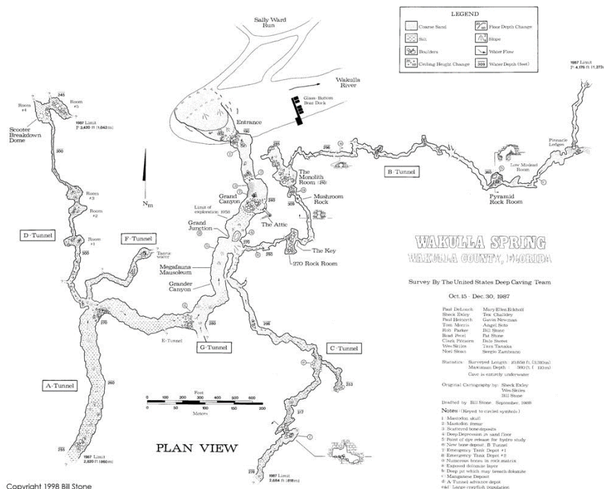
Wakulla Springs cave system map (Bill Stone, 1988)
