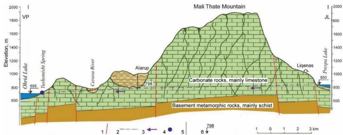
Hydrogeological cross-section between lakes Ohrid and Prespa. Legend: 1 tectonic fault; 2 groundwater level; 3 groundwater flow direction; 4 karts spring; 5 boreholes, 6. Groundwater level (m a.s.l.)
