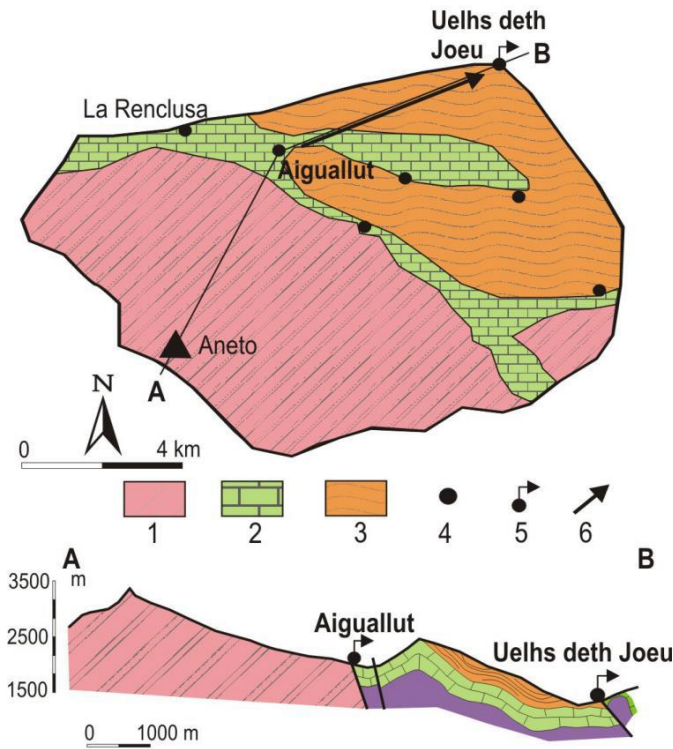
Hydrogeological section of the Aiguallut (swallet)-Uelhs deth Joeu (spring) system. Lithologies: 1) Hercinian granites, 2) Devonian limestones and 3) Carboniferous metapelites. Symbols: 4) swallowt, 5) karst spring and 6) preferential groundwater flows (modified from Freixes, 2014).
