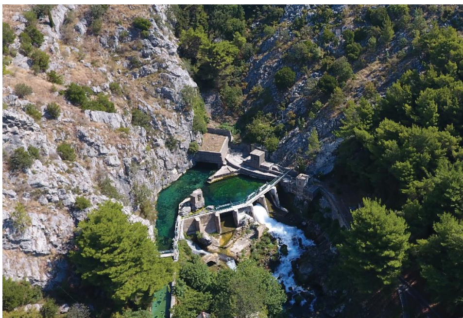
The water intake structures at the Jadro River's spring (photo: M. Žabčič)
