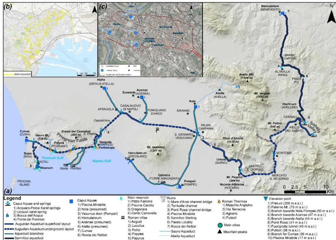
Layout of Roman Aqueducts tapped Serino springs (from Esposito et al., 2025-modified)
