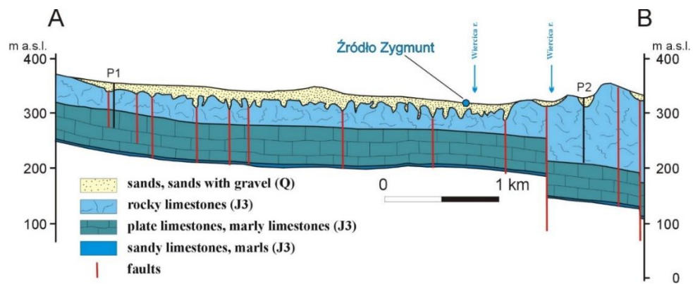
Geological cross – section with the location of the spring (after R. Więkowski, 1973)
