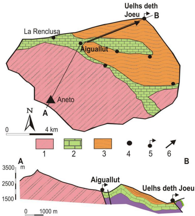
Hydrogeological section of the Aiguallut (swallet)-Uelhs deth Joeu (spring) system. Lithologies: 1) Hercinian granites, 2) Devonian limestones and 3) Carboniferous metapelites. Symbols: 4) swallow, 5) karst spring and 6) preferential groundwater flows (modified from Freixes, 2014).
