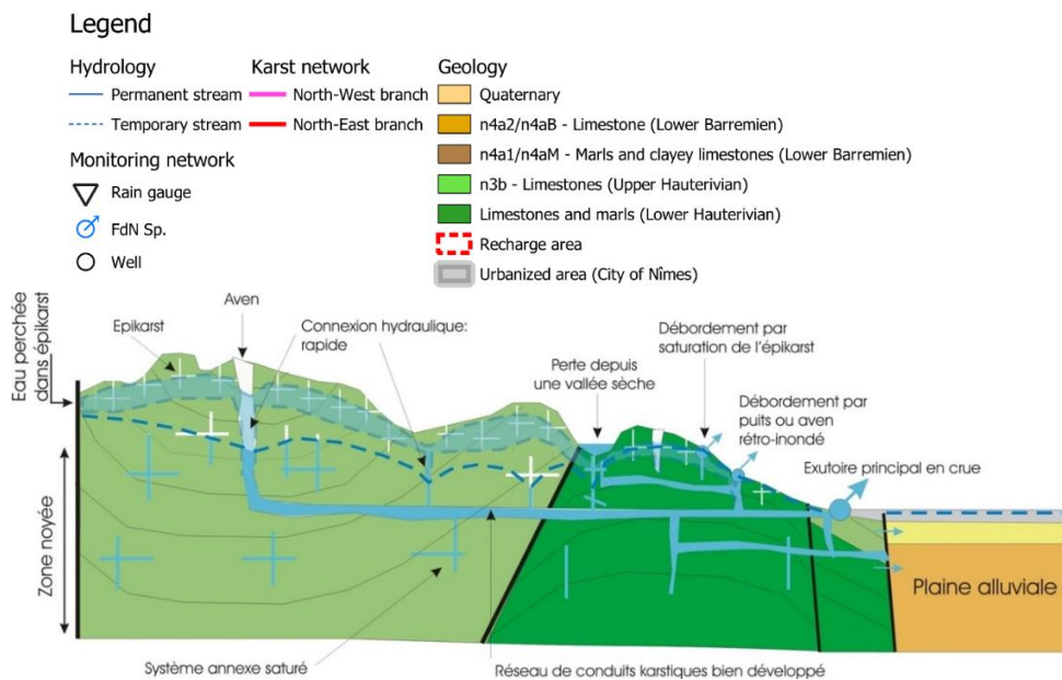
Hydrogeological conceptual model of Fontaine de Nîmes karst system during flood events (Maréchal et al., 2005).
